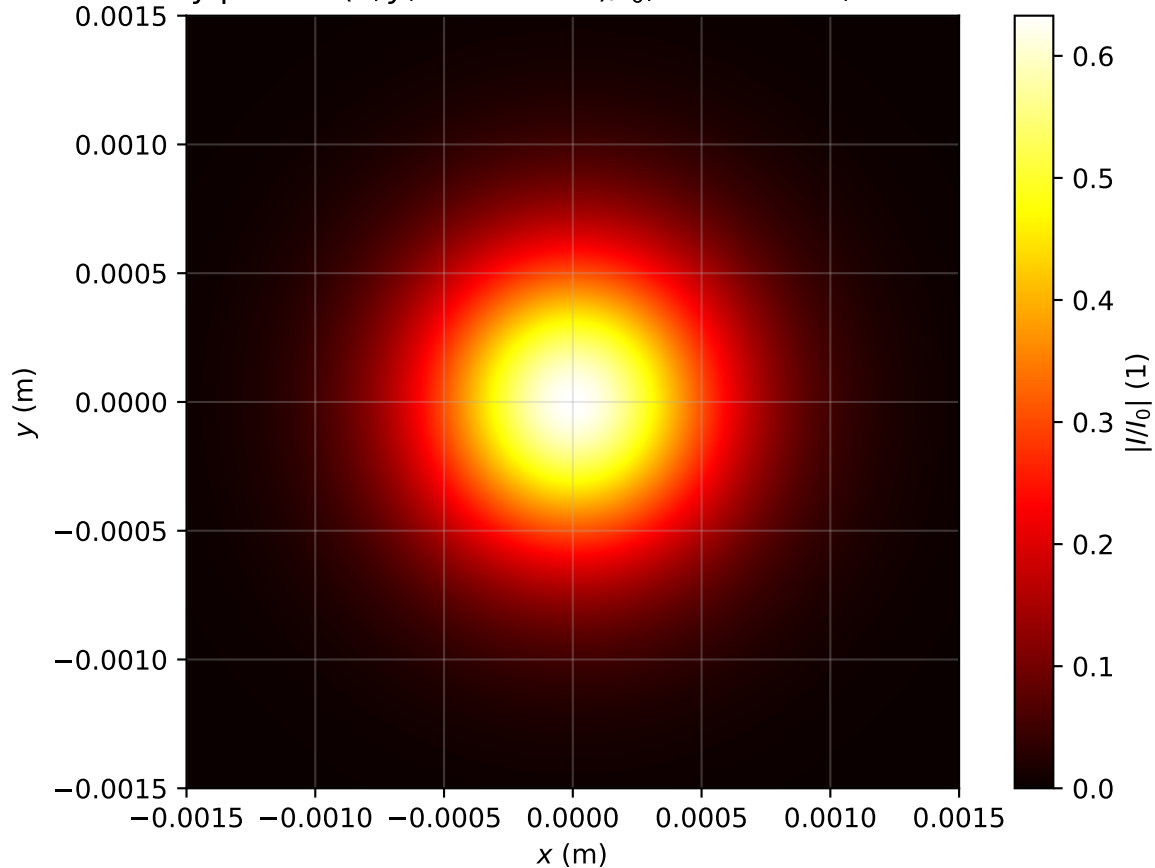
Intensity profile I(x, y, z = 2.707m)/I_0 , Pin=0.5Pcr, artificial time
